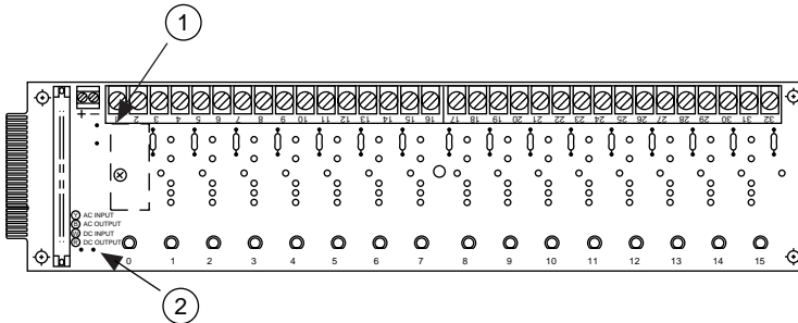
Figure 1. Grayhill 8 Module Backplane Jumper Locations
